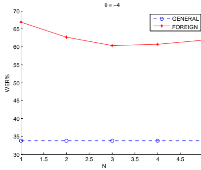
Figure 2: WERs on the two test sets. N is the number of referral high-frequency Chinese words. The value of \theta is -4 .
