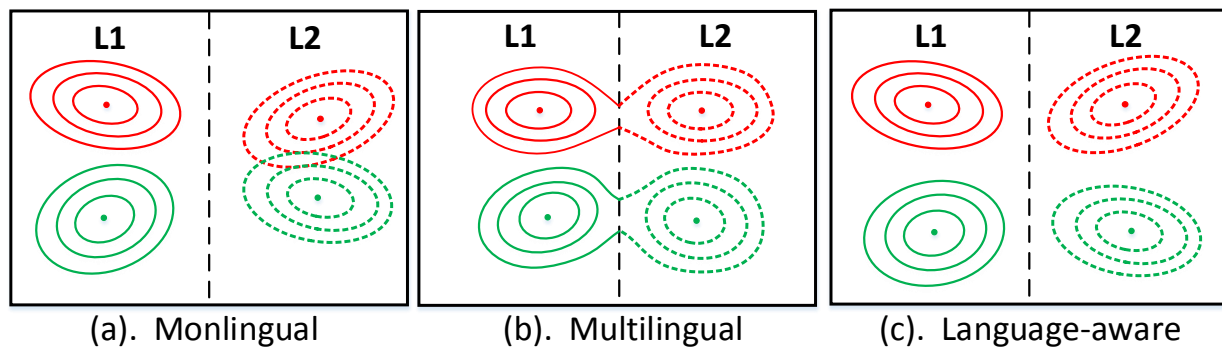
Fig. 1. Distribution of latent speaker factors with PLDA different training methods.
